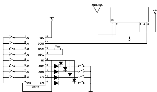
Figure 3: QFMT6 Quasar Transmitter Application Circuit
