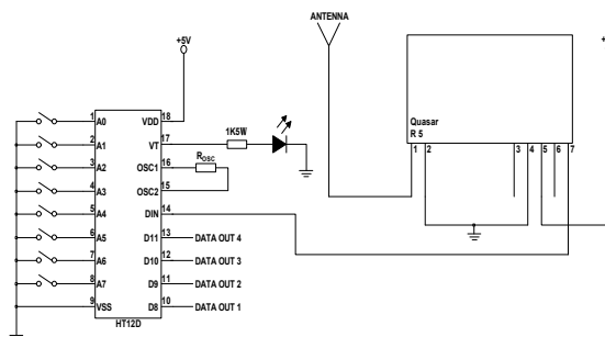
Figure 4: QFMR6 Quasar Receiver Application Circuit
